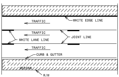
MARKING PLACEMENT DETAIL
